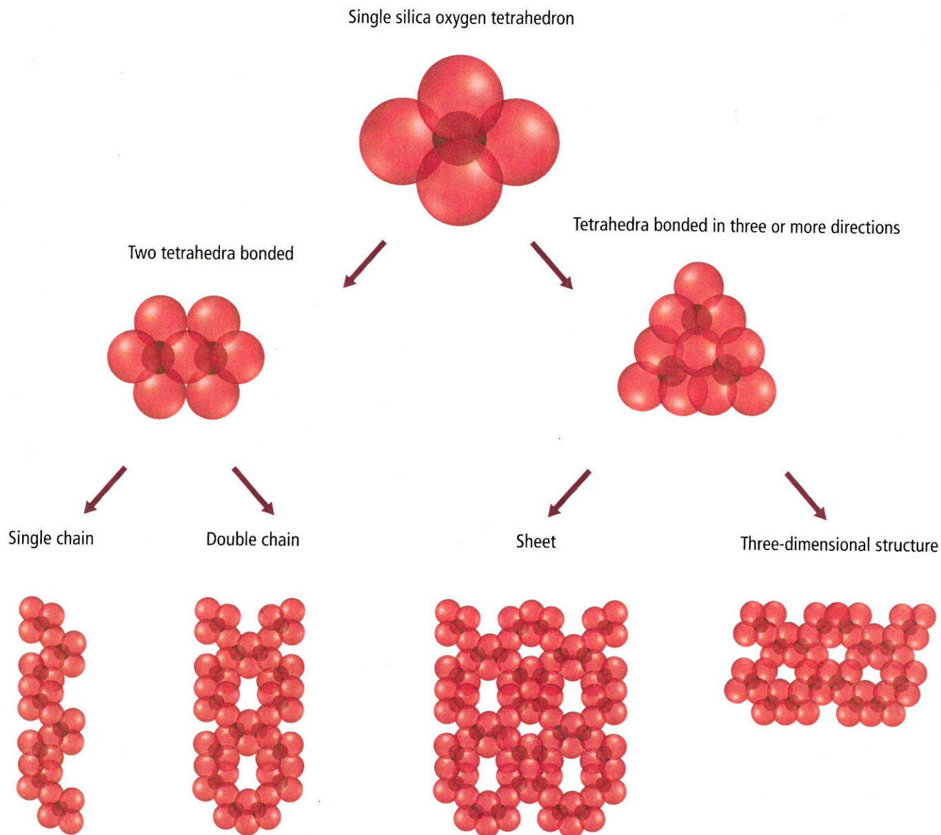
Figure 4.13 The tetrahedron formed by silicates contains four oxygen ions bonded to a central silicon atom. Chains, sheets, and complex structures form as the tetrahedra bond with other tetrahedra. These structures become the numerous silicate minerals that are present on Earth.
